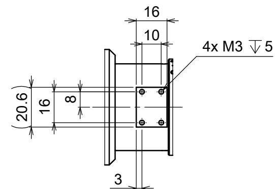
VIEW A
