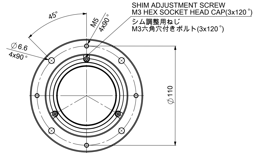
VIEW A MOUNTING PORTION DETAIL VIEW フランジ取付部詳細
