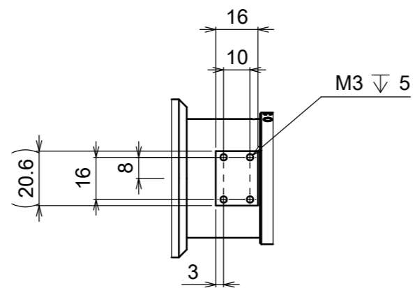
VIEW A
