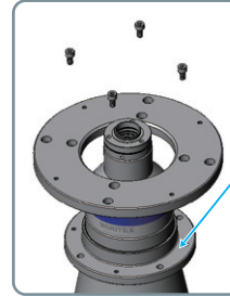
Flange Adapter MTL-FA** (Option)
